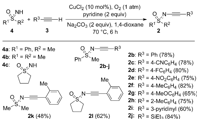
Scheme 2. Substrate scope of the oxidative N-alkynylation.
